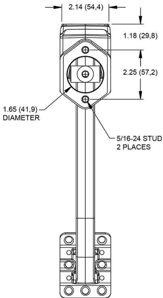
FOOT PAD DETAIL
